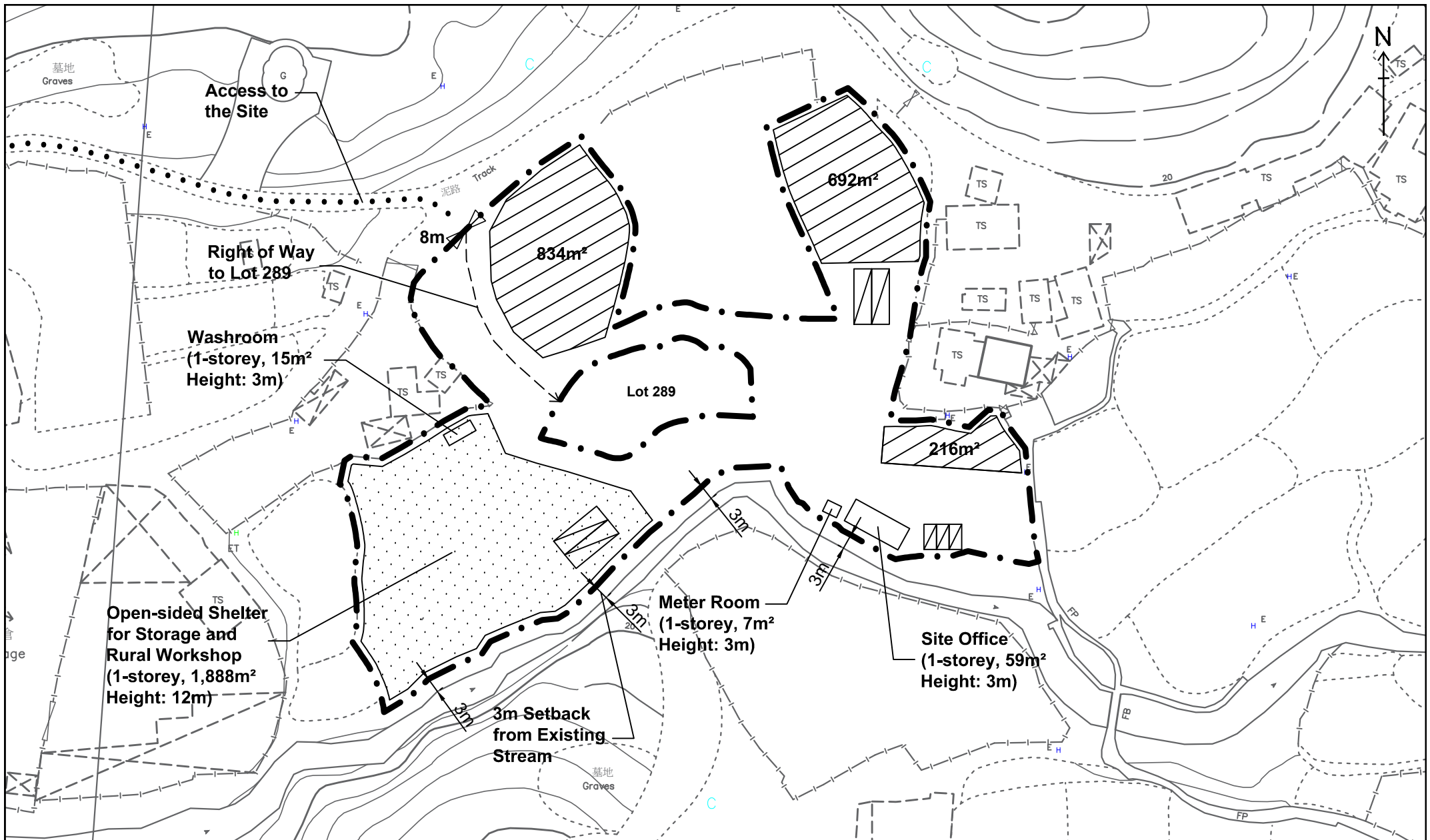
Figure 4 Layout Plan
